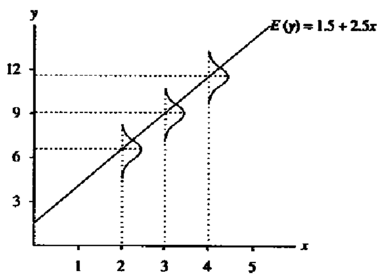
FIGURE 11.2 Theoretical distribution of y in regression
